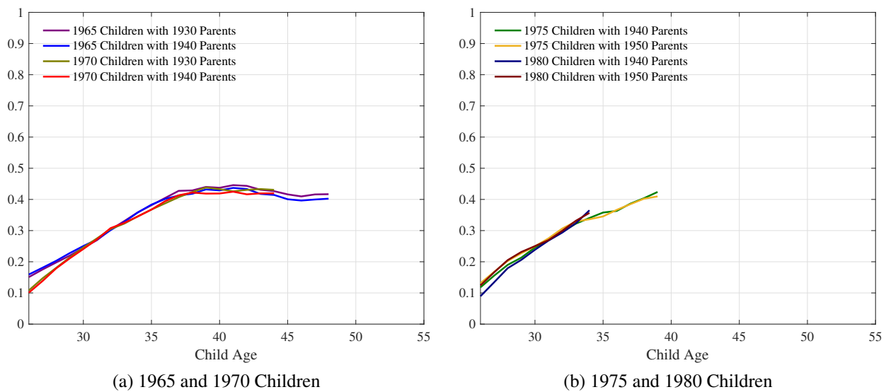
Figure 9: \text{Var}(\theta_{k,t})/\text{Var}(y_{k,t})
