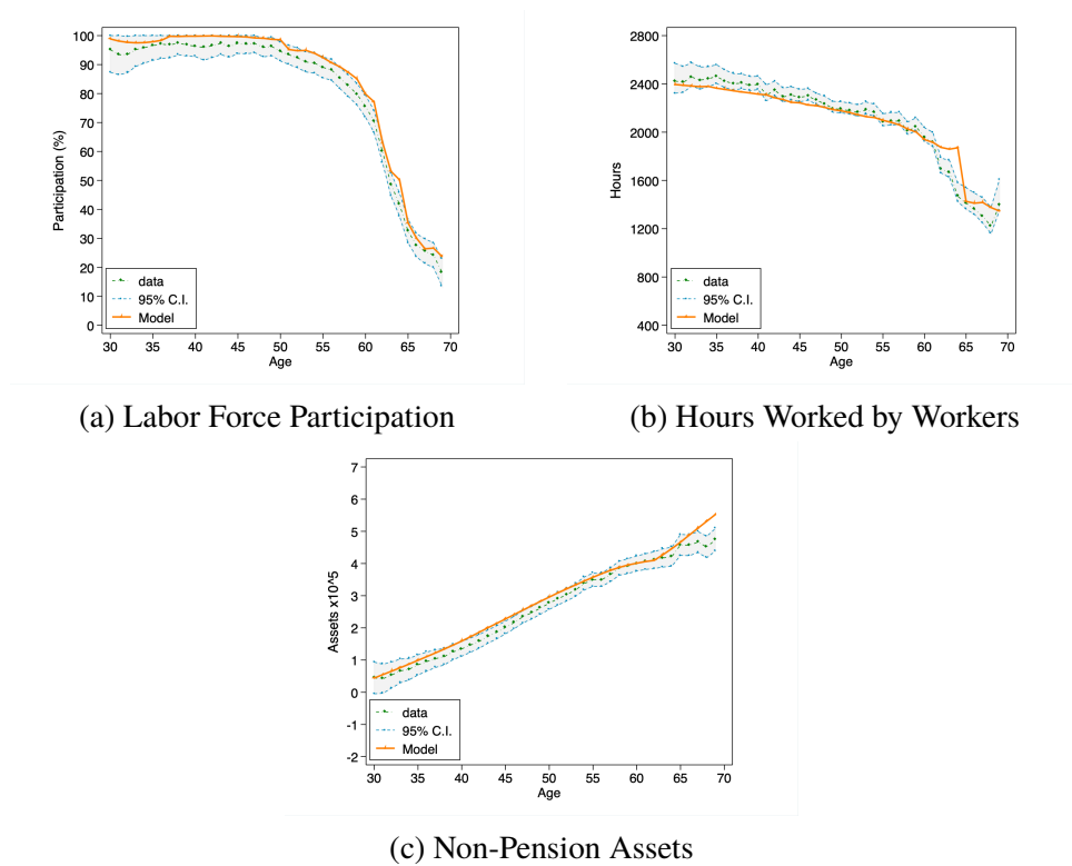
Fig. 9. Model v.s. Data Profiles: Untargeted Moments
